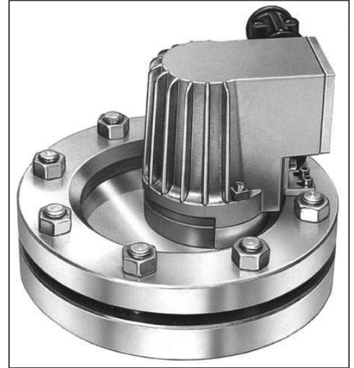
EX-light fitting KEL mounted on circular sight glass to DIN 28120
